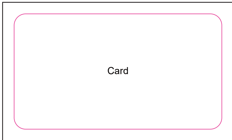
— Knife line Card size: 90mm(W) x 50mm(H) Shown at 100% actual size
